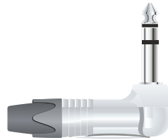
3 pole right-angle 1/4" professional phone plug, nickel contacts, nickel shell / NP3RX
